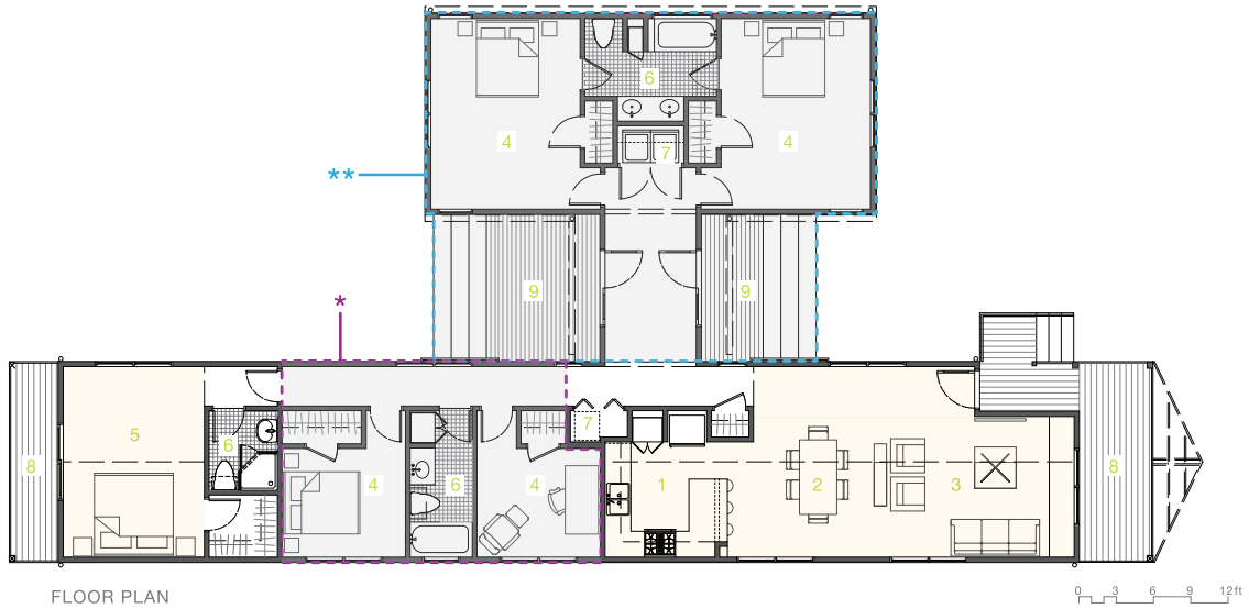
FLOOR PLAN
